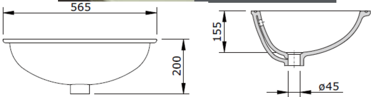
Sanindusa — Vouga Under Counter Basin Model No.— 108350
