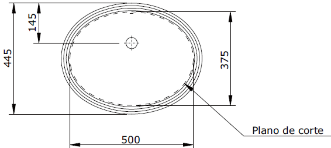
Sanindusa — Vouga Under Counter Basin Model No.— 108350
