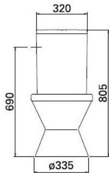
112111 tanque cisterna cistern reservoir
