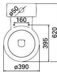
112022 sanita compacta d/p inodoro cisterna baja s/h wc bowl monobloc p-trap cuvette s/h
