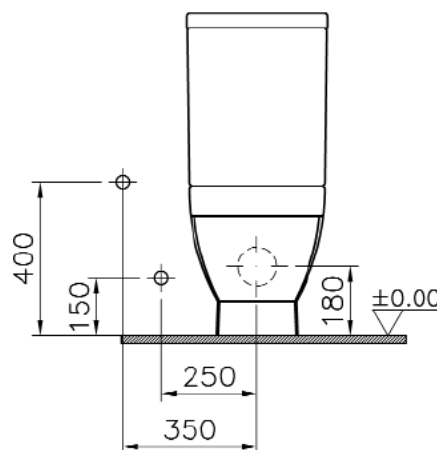
Standard connection
