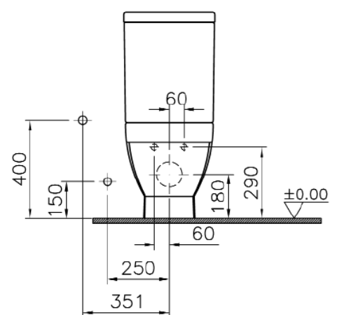
Concealed connection
