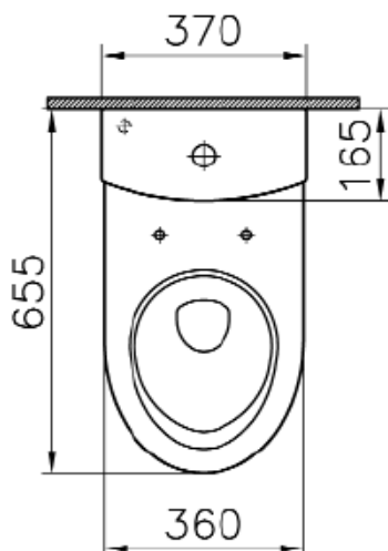
Standard connection
