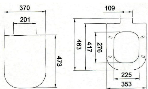
55-003-009 Soft Closing Seat & Cover
