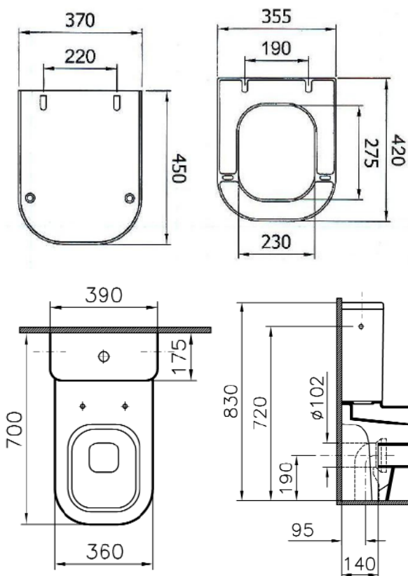
35-003-001 Seat & Cover
