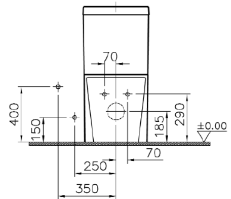
Concealed connection
