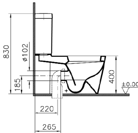
Standard connection
