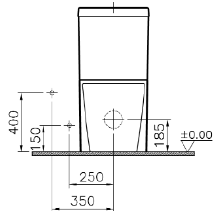
Standard connection
