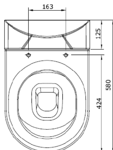
Model : 104012 Product : Floor Stand W.C. Pan (P-Trap)
