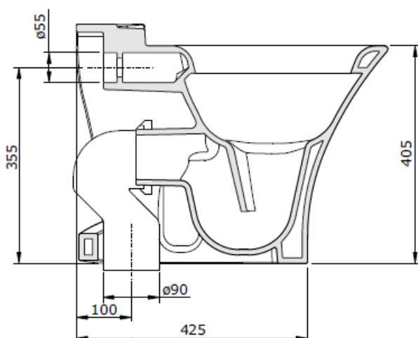
Model : 104011 Product : Floor Stand W.C. Pan (S-Trap)
