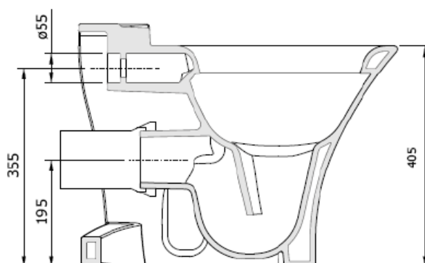
Model : 104012 Product : Floor Stand W.C. Pan (P-Trap)
