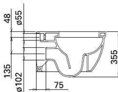
Product : Wall Hung WC Model : 106032
