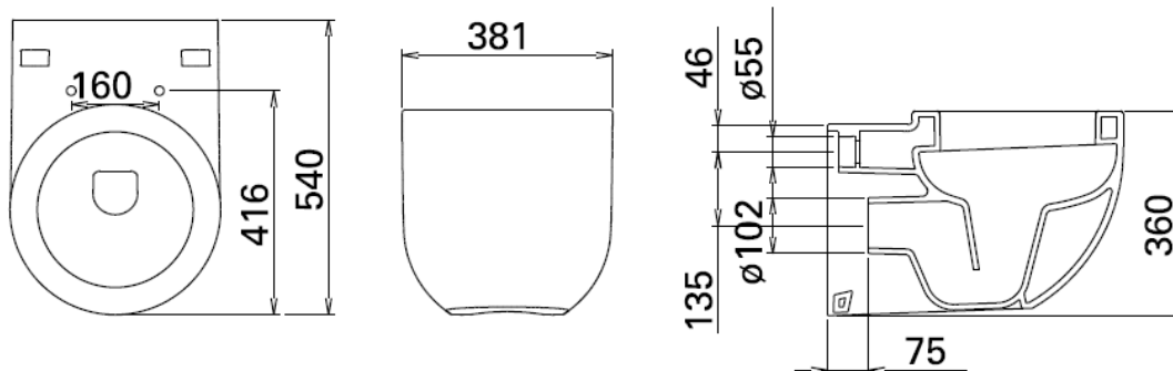
Product : Wall Hung WC Model : 111032
