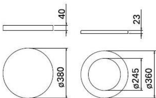
Product : Toilet Seat & Cover Model : 21111
